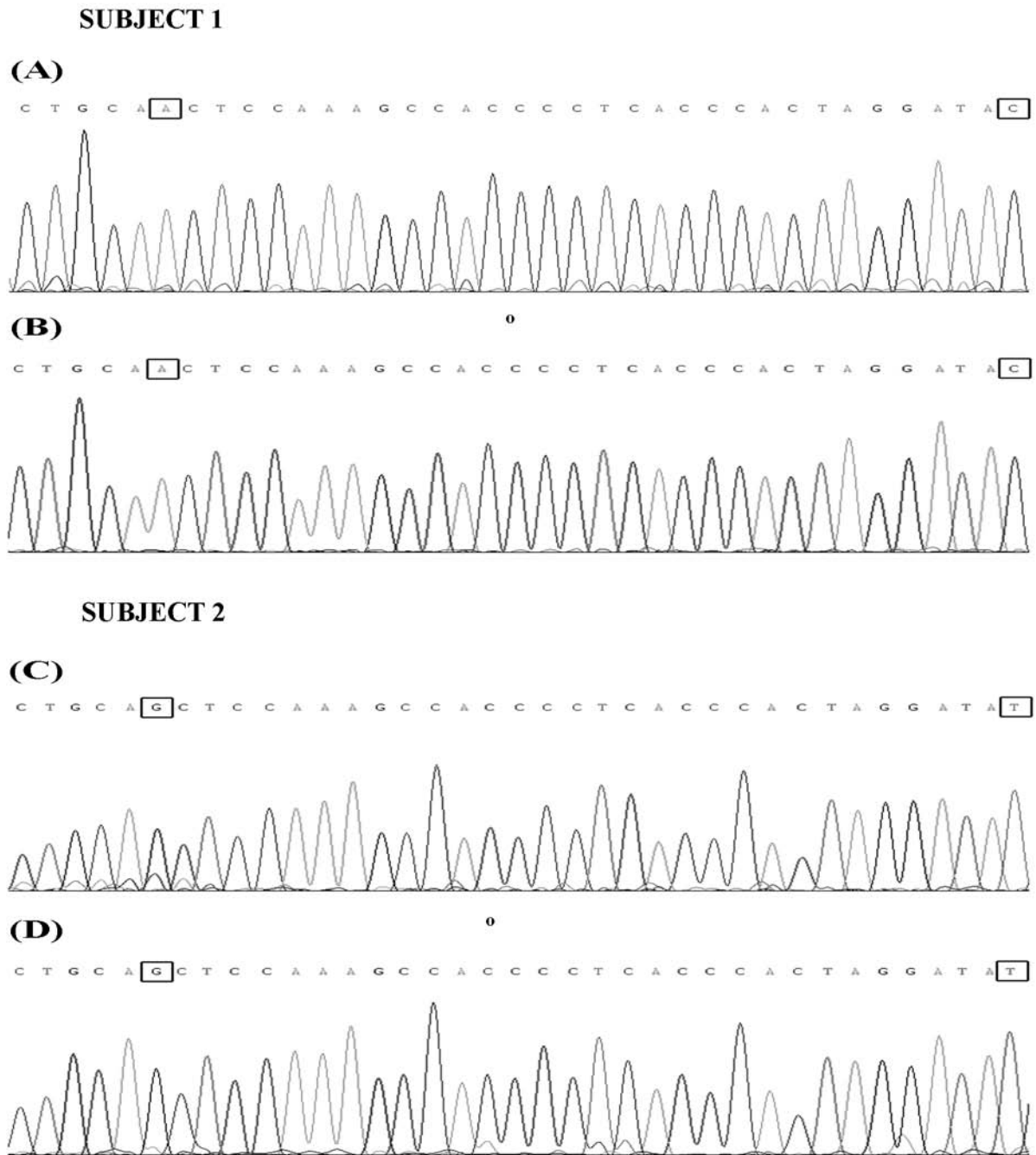
Fig. 3. Part of the mtDNA HVSI sequence. (A) and (C) - sequences from PCR products amplified on genomic DNA; (B) and (D) - sequences from PCR products amplified directly from buccal cells. (A) and (B) – Subject 1; (C) and (D) – Subject 2; Boxed nucleotides represent single nucleotide polymorphisms (SNPs) detected within the HVSI region of analyzed subjects.
