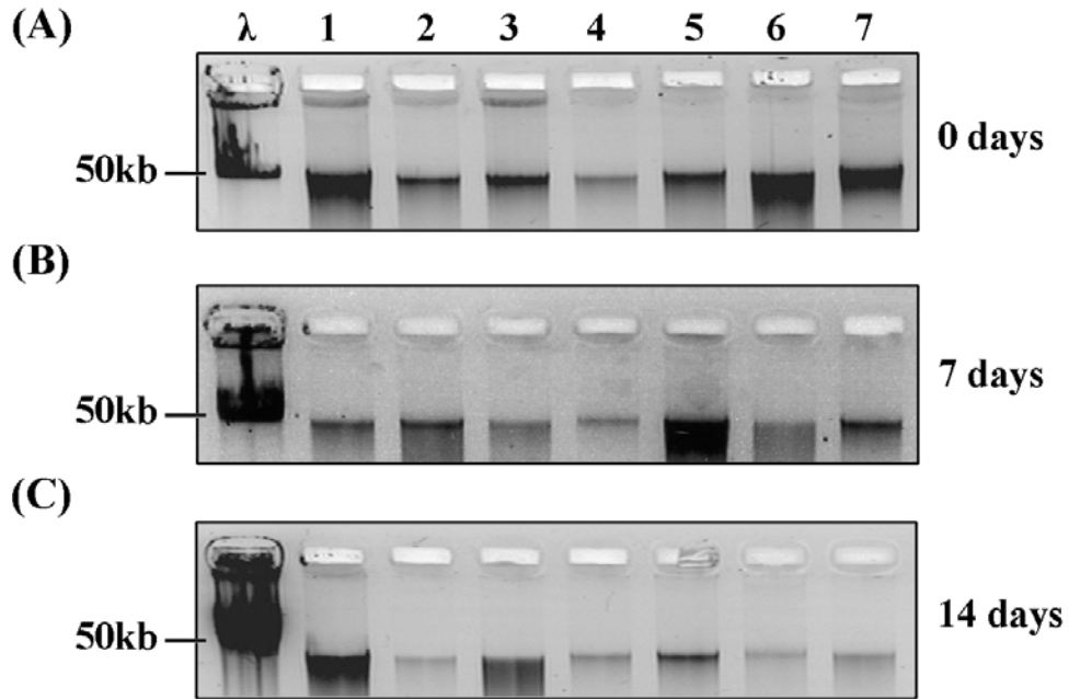
Fig. 1. Electrophoretic analysis of genomic DNA extracted from buccal cells collected from swabs that were processed immediately (A), after 7 days at room temperature (B), or after 14 days at room temperature (C). Lane \lambda : molecular weight marker \lambda DNA; Lanes 1-7: genomic DNA extracted from buccal cells.
