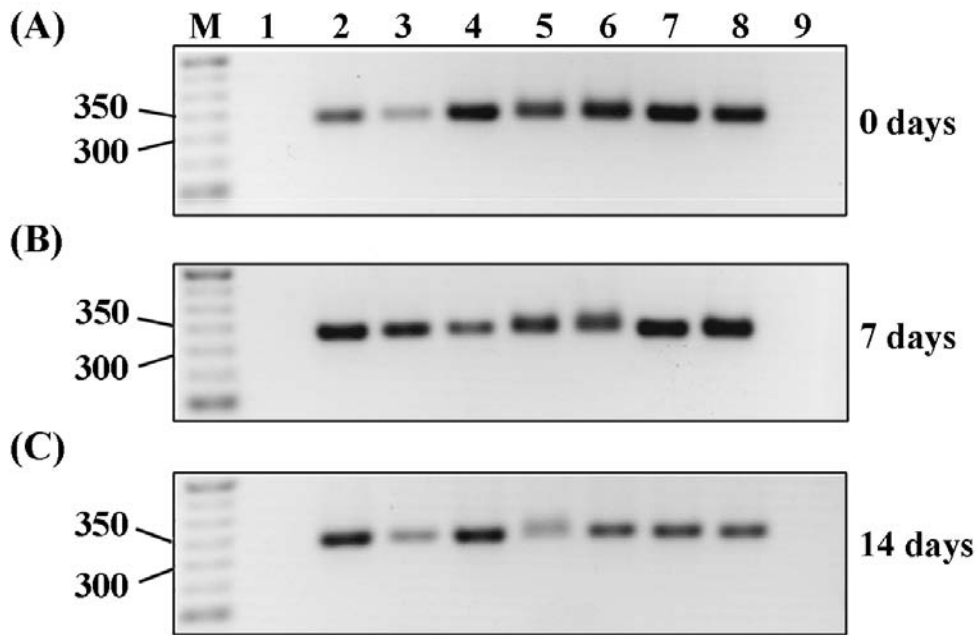
Fig. 2. The effect of long-term storage of buccal swabs at room temperature on direct PCR amplification. A 330 bp fragment of the HVSI region was amplified directly from the buccal cells collected from swabs that were processed immediately (A), after 7 days at room temperature (B) or after 14 days at room temperature (C). Lane M: O'RangeRuler™ 50 bp DNA Ladder (Fermentas); Lanes 1 and 9: negative PCR controls; Lanes 2-8: direct PCR products from buccal cells.
