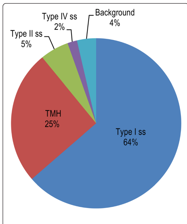
Figure 2 Types of membrane-targeting signals detected in metasecretome pilot library ORFs. Abbreviations used for membrane-targeting signal types: ss, signal sequence; Type I ss, classical ss; Type II ss, lipoprotein ss; Type IV ss, pilin-like ss; TMH, N-terminal or internal transmembrane \alpha helix/helices; background - ORFs without membrane-targeting signal or shorter than 24 amino acids.
